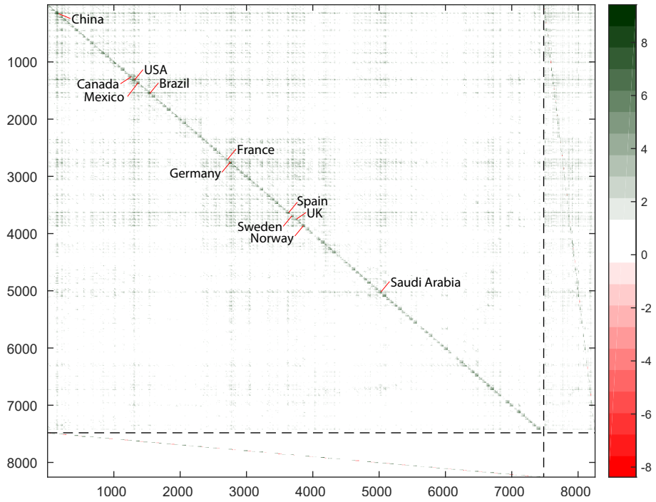
Fig. 4: Basic-price MRIO sheet in the regional and sectoral classification of the 2011 GTAP9 database (GTAP 2016), for the year 2013. Colour scaling as in Fig. 2.
