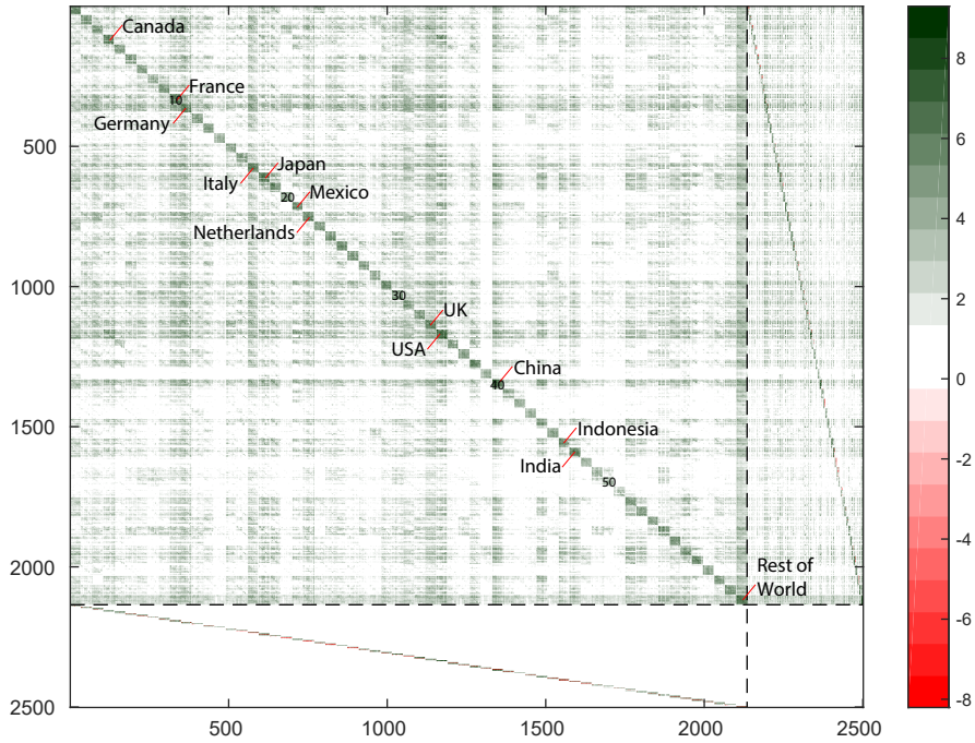
Fig. 2: Basic-price MRIO sheet in the regional and sectoral classification of the 2011 OECD Inter-Country Input-Output (ICIO) Tables (OECD 2015), for the year 2013. Colours are scaled as \text{sgn}(x) \log_{10}(|x|) , with x expressed in current US$, so that levels 6 and -6 correspond to transactions of 1 million and -1 million US$, respectively.
