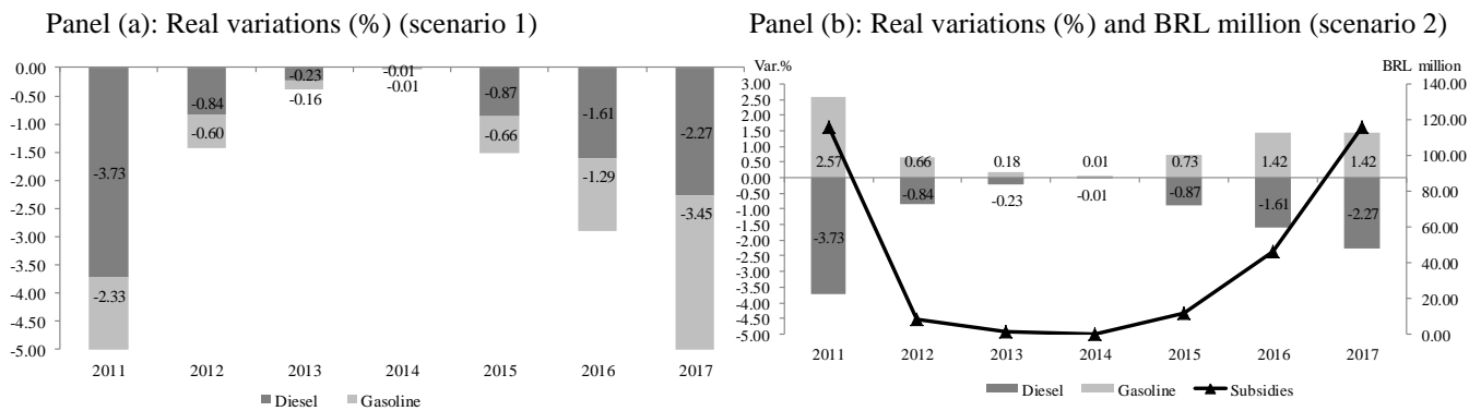
Figure 4 – Policy shocks
